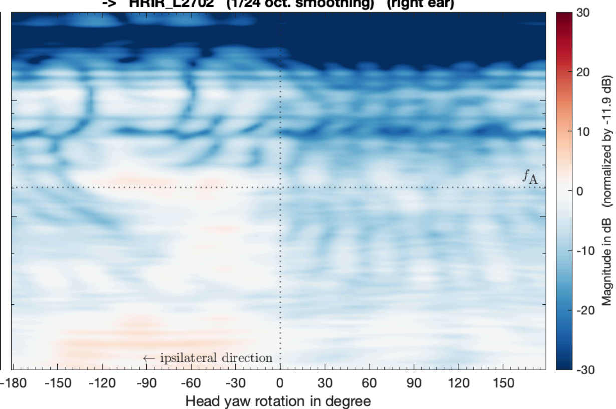
LBS_VSA_EMA17_PAC_struct_SubSampled_SH29 -> HRIR_L2702 (1/24 oct. smoothing) (right ear)
