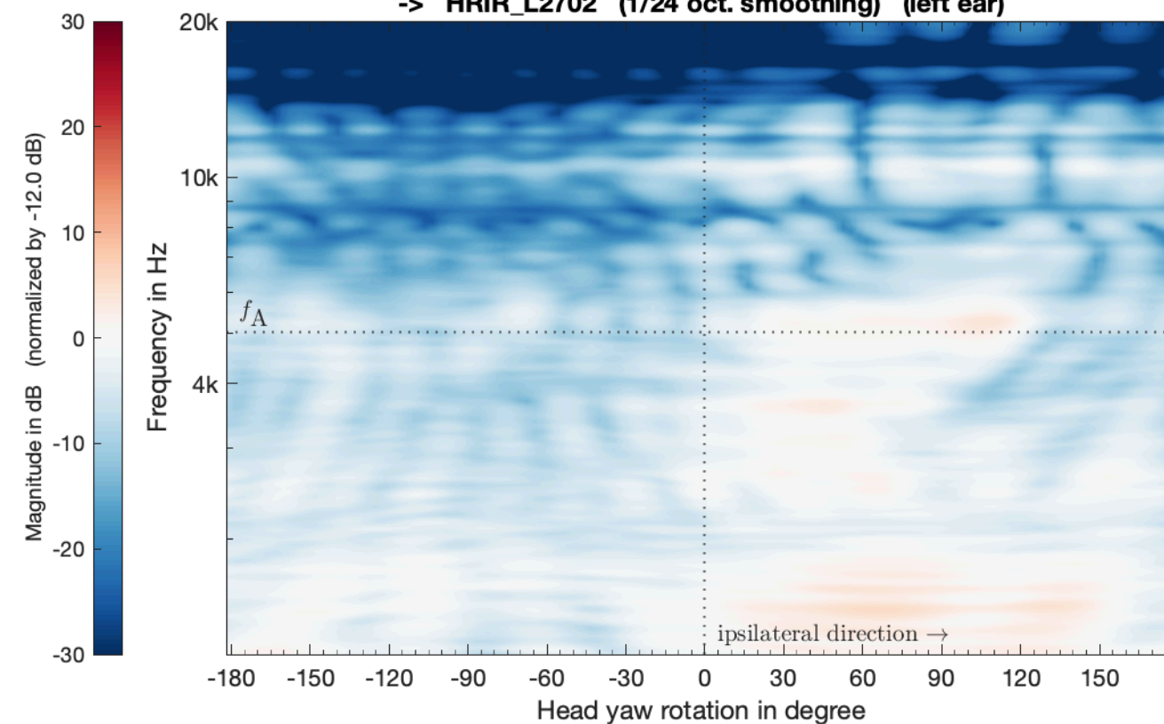
LBS_VSA_EMA17_PAC_struct_SubSampled_SH29 -> HRIR_L2702 (1/24 oct. smoothing) (left ear)
