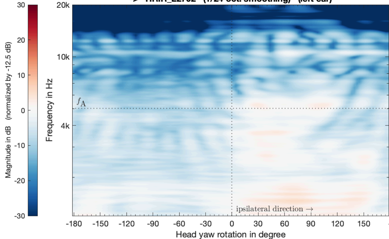
LBS_VSA_EMA17_PAC_struct_SubSampled_SH29_eMagLS -> HRIR_L2702 (1/24 oct. smoothing) (left ear)
