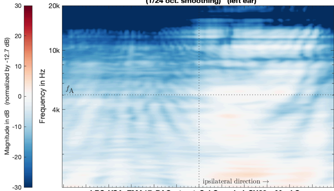
LBS_VSA_EMA17_PAC_struct_SubSampled_SH29_eMagLS -> HRIR_L2702 (1/24 oct. smoothing) (left ear)
