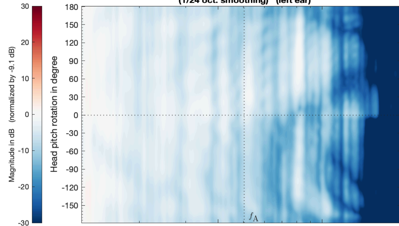
LBS_VSA_EMA17_PAC_struct_SubSampled_SH29_vertical -> HRIR_L2702 (1/24 oct. smoothing) (left ear)
