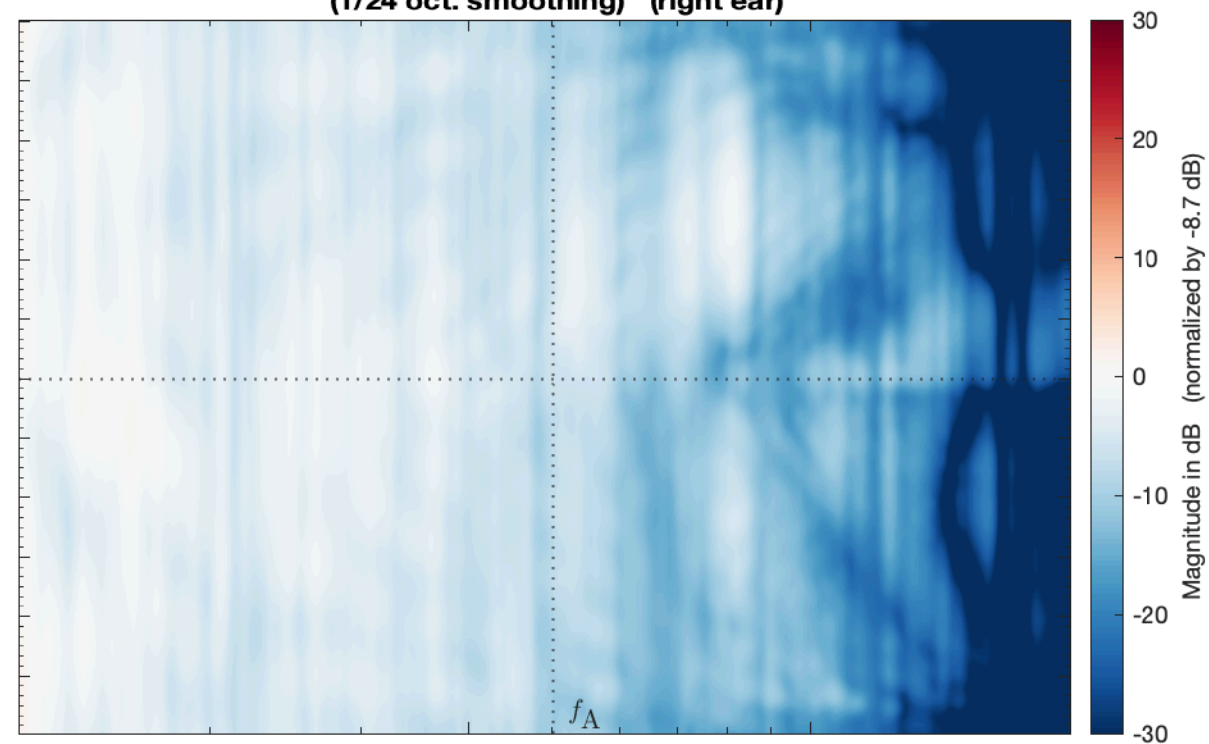
LBS_VSA_EMA17_PAC_struct_SubSampled_SH29_vertical -> HRIR_L2702 (1/24 oct. smoothing) (right ear)
