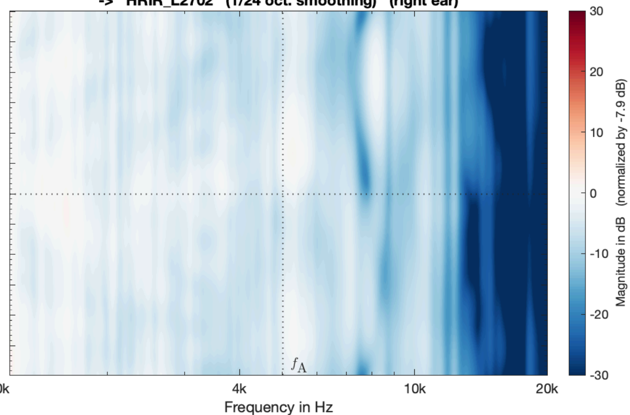
LBS_VSA_EMA17_PAC_struct_SubSampled_SH29_vertical -> HRIR_L2702 (1/24 oct. smoothing) (right ear)
