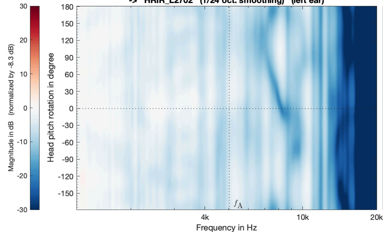
LBS_VSA_EMA17_PAC_struct_SubSampled_SH29_vertical -> HRIR_L2702 (1/24 oct. smoothing) (left ear)
