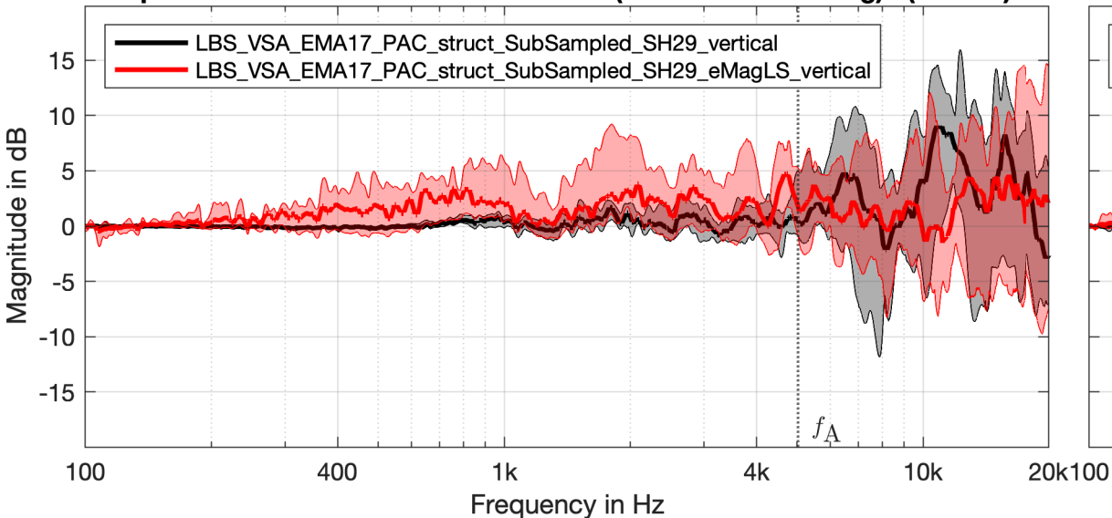
Spectral difference to BRIR reference (1/24 oct. smoothing) (ears average)
