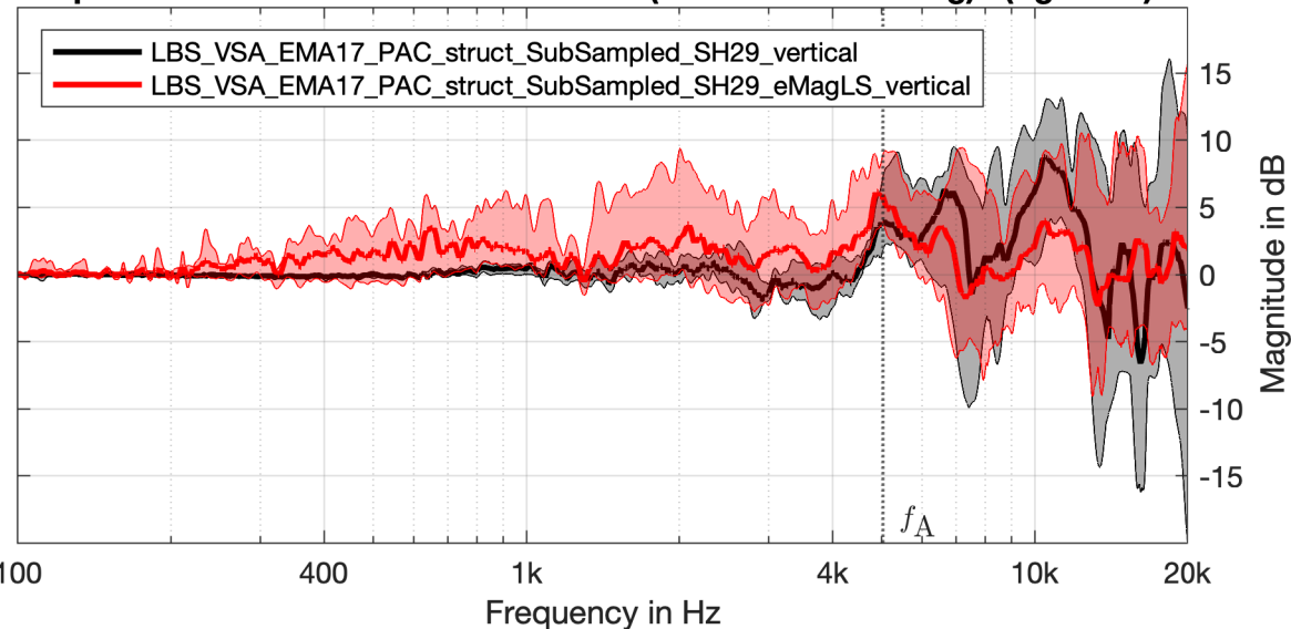
Spectral difference to BRIR reference (1/24 oct. smoothing) (right ear)
