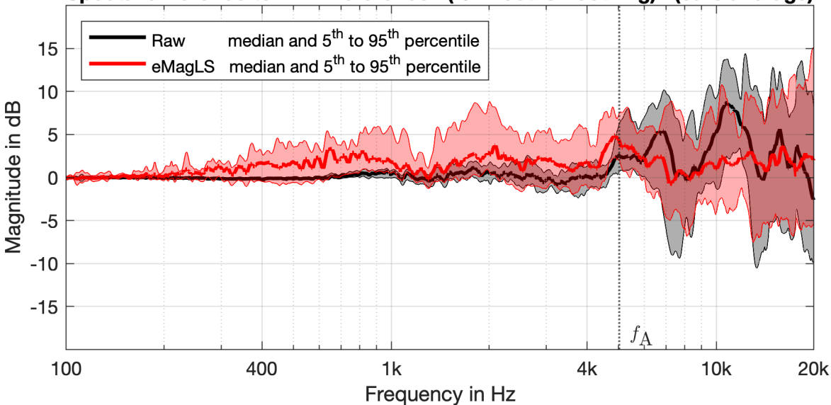
Spectral difference to BRIR reference (1/24 oct. smoothing) (ears average)
