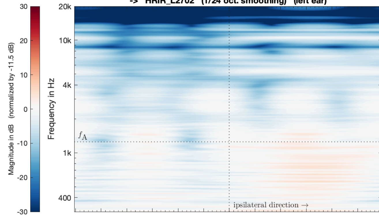
LBS_VSA_EMA5_PAC_struct_SubSampled_SH29 -> HRIR_L2702 (1/24 oct. smoothing) (left ear)
