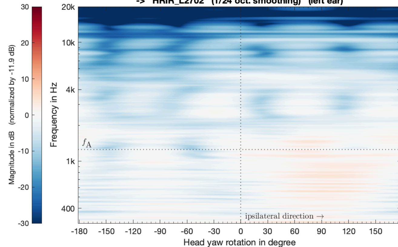
LBS_VSA_EMA5_PAC_struct_SubSampled_SH29_eMagLS -> HRIR_L2702 (1/24 oct. smoothing) (left ear)
