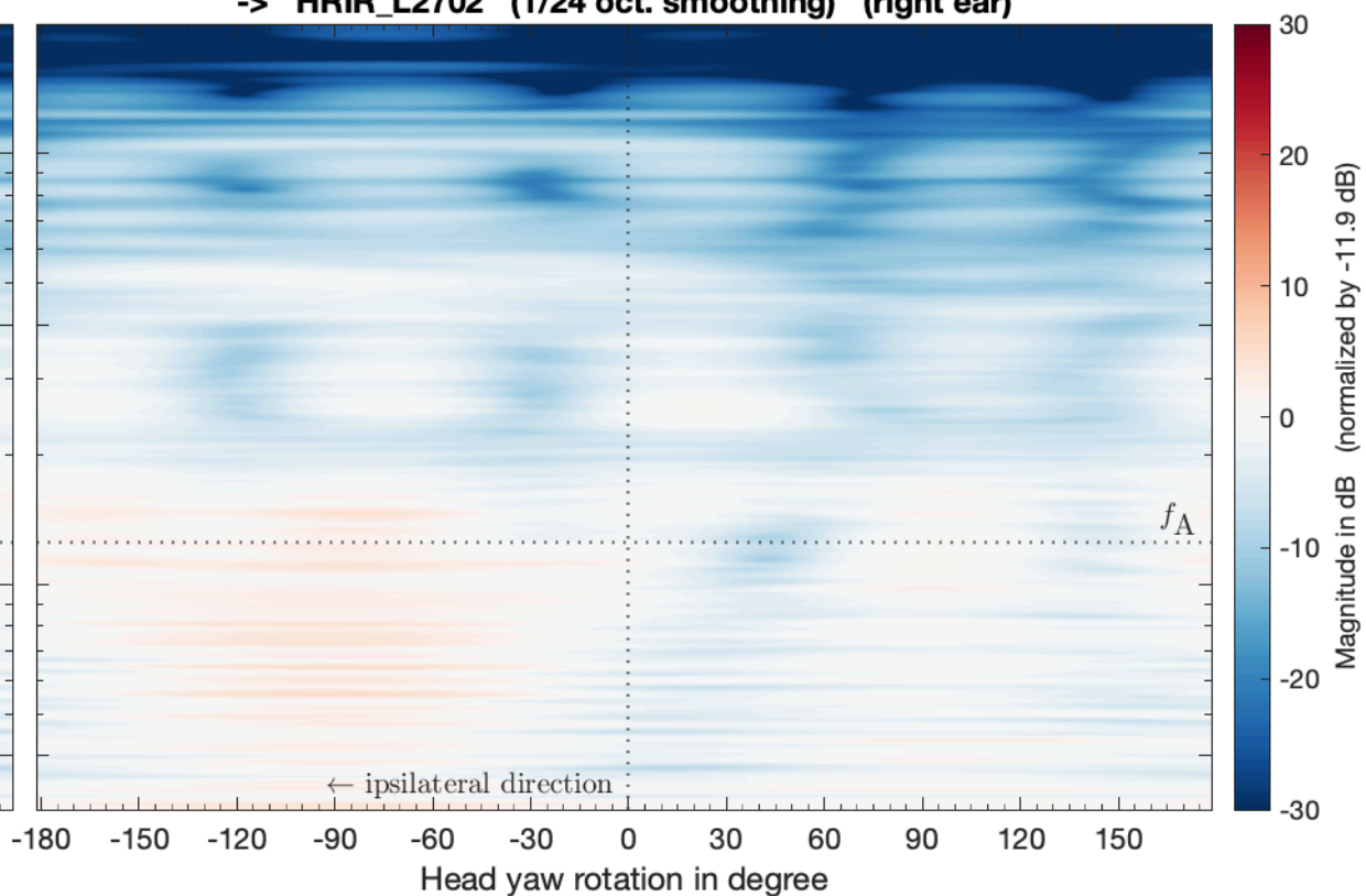
LBS_VSA_EMA5_PAC_struct_SubSampled_SH29_eMagLS -> HRIR_L2702 (1/24 oct. smoothing) (right ear)
