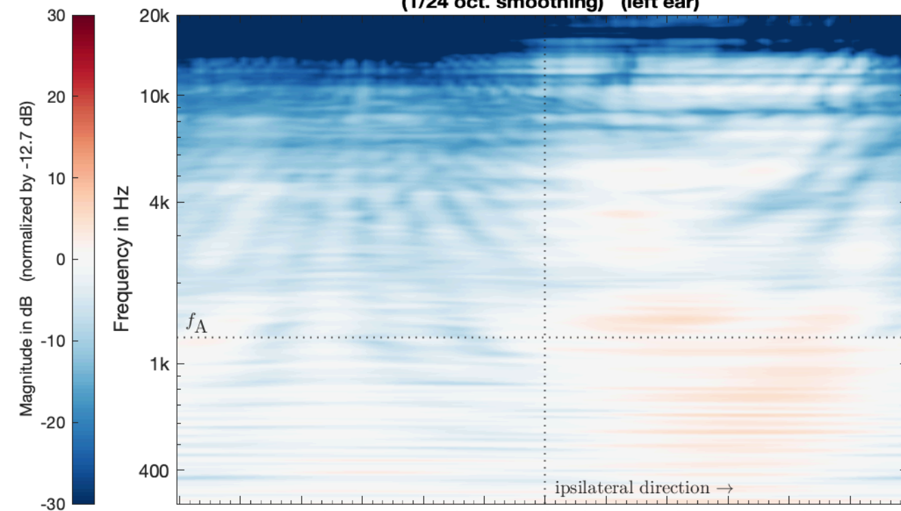
LBS_VSA_EMA5_PAC_struct_SubSampled_SH29_eMagLS -> HRIR_L2702 (1/24 oct. smoothing) (left ear)
