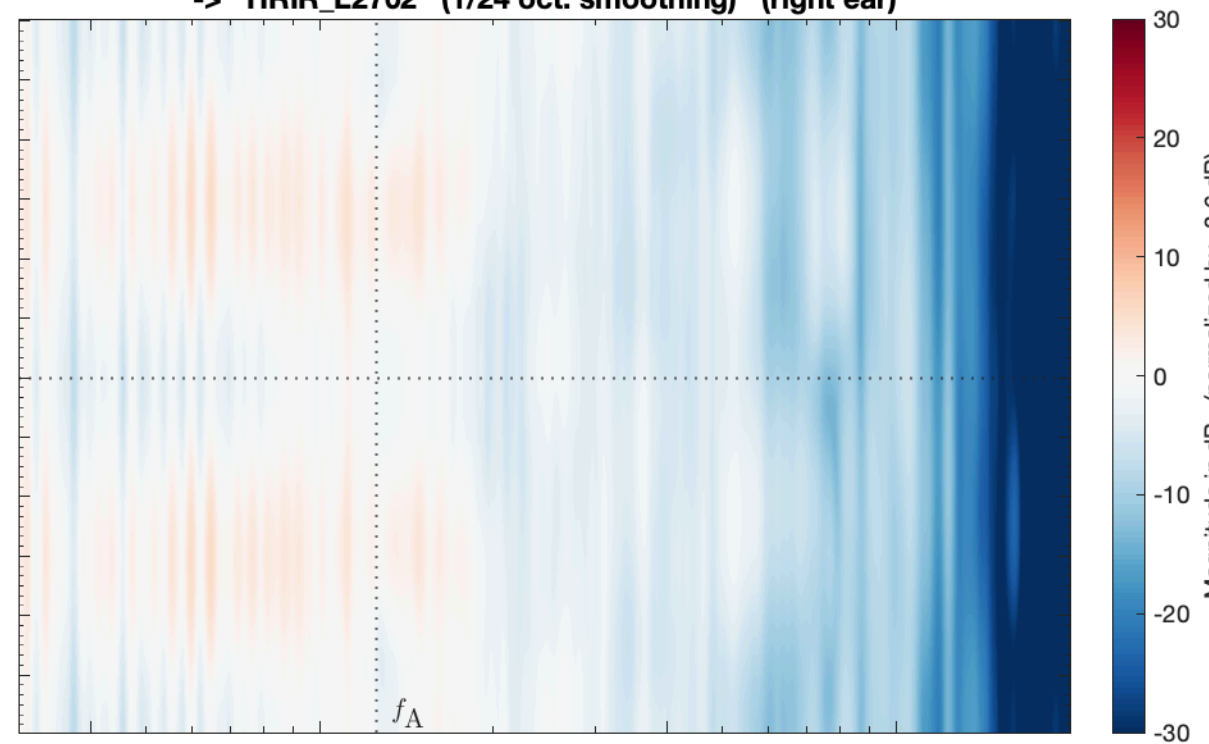
LBS_VSA_EMA5_PAC_struct_SubSampled_SH29_eMagLS_vertical -> HRIR_L2702 (1/24 oct. smoothing) (right ear)
