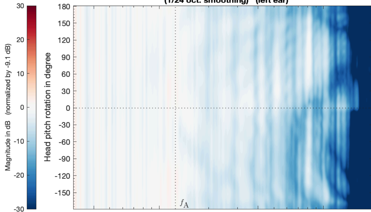
LBS_VSA_EMA5_PAC_struct_SubSampled_SH29_eMagLS_vertical -> HRIR_L2702 (1/24 oct. smoothing) (left ear)
