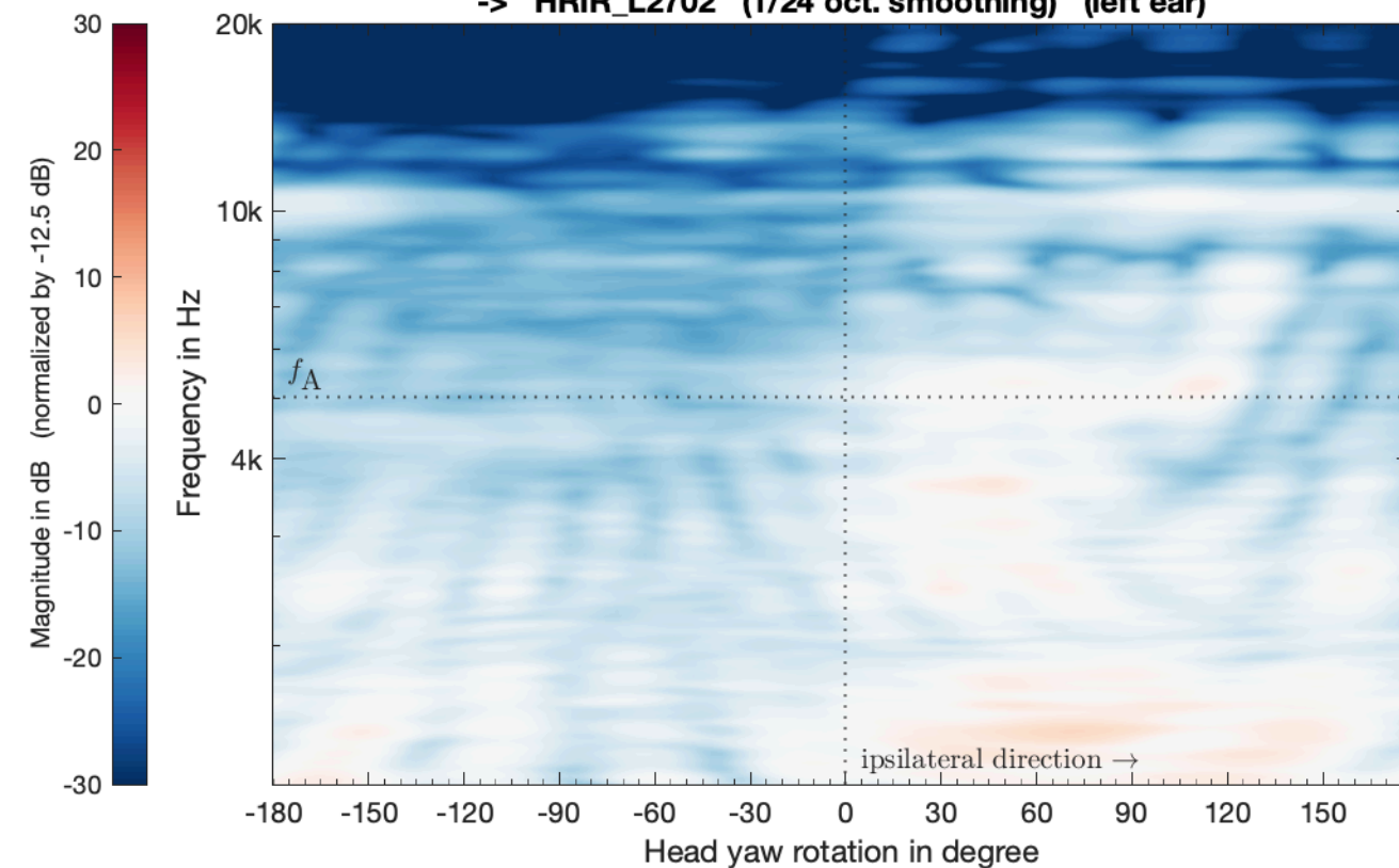
LBS_VSA_SMA_TD146_PAC_struct_SubSampled_SH29_eMagLS -> HRIR_L2702 (1/24 oct. smoothing) (left ear)
