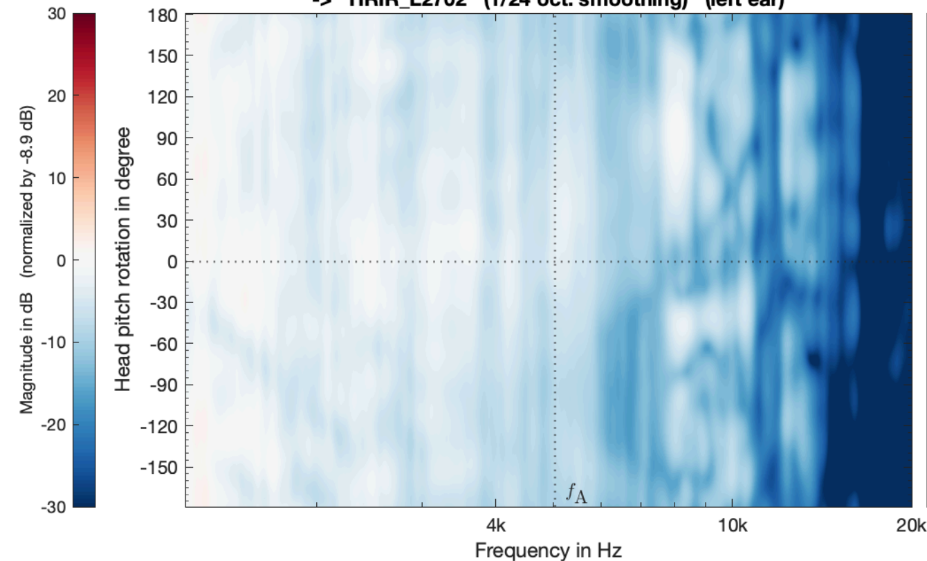
LBS_VSA_SMA_TD146_PAC_struct_SubSampled_SH29_eMagLS_vertical -> HRIR_L2702 (1/24 oct. smoothing) (left ear)
