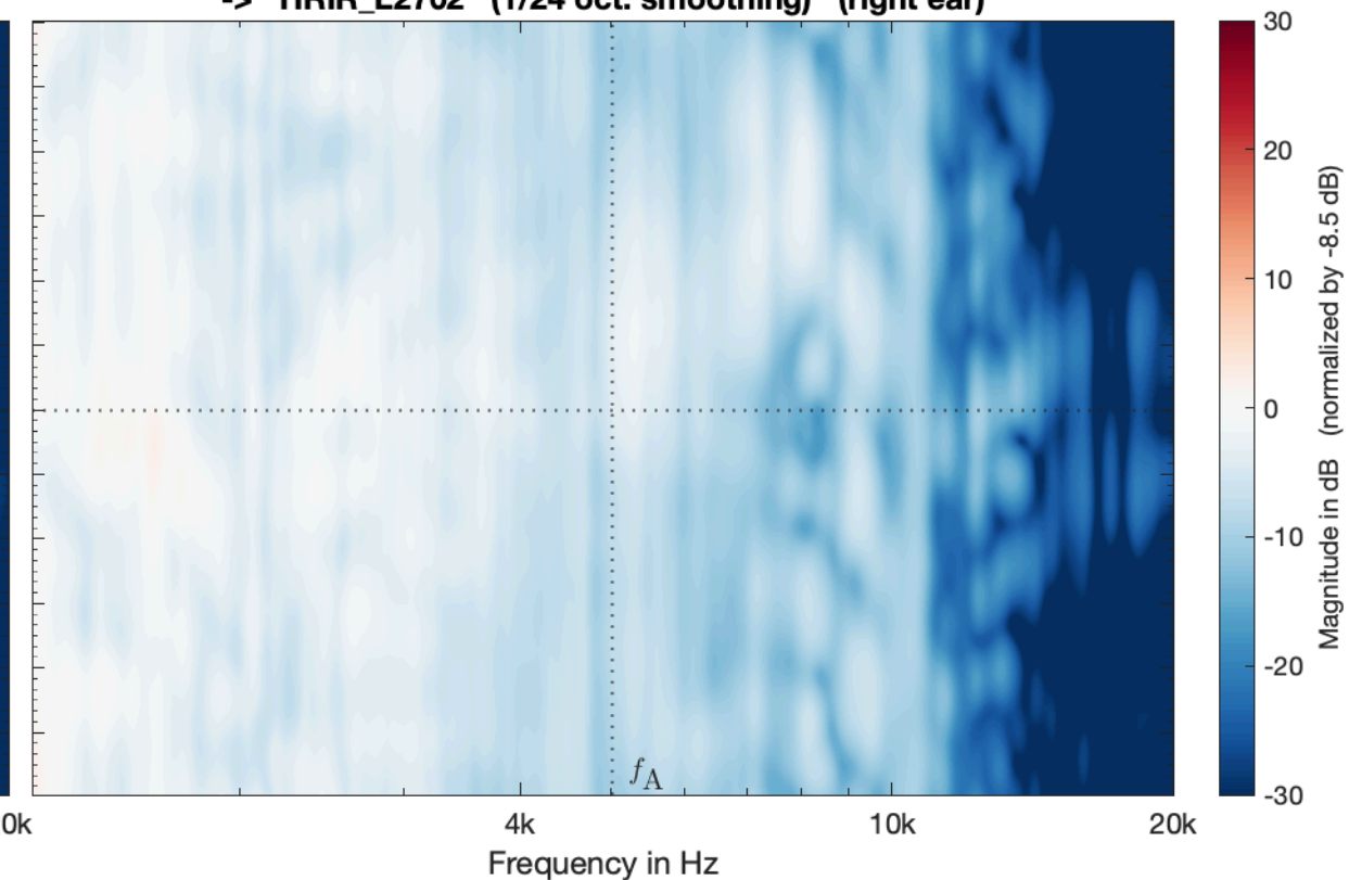
LBS_VSA_SMA_TD146_PAC_struct_SubSampled_SH29_eMagLS_vertical -> HRIR_L2702 (1/24 oct. smoothing) (right ear)
