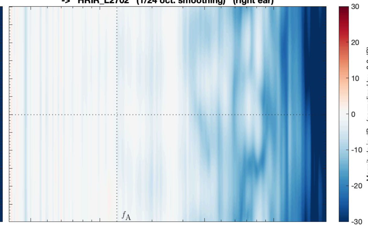
LBS_VSA_SMA_TD14_PAC_struct_SubSampled_SH29_eMagLS_vertical -> HRIR_L2702 (1/24 oct. smoothing) (right ear)
