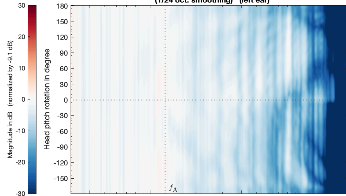
LBS_VSA_SMA_TD14_PAC_struct_SubSampled_SH29_vertical -> HRIR_L2702 (1/24 oct. smoothing) (left ear)
