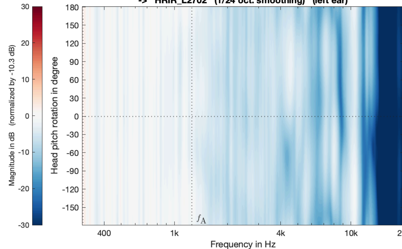
LBS_VSA_SMA_TD14_PAC_struct_SubSampled_SH29_vertical -> HRIR_L2702 (1/24 oct. smoothing) (left ear)
