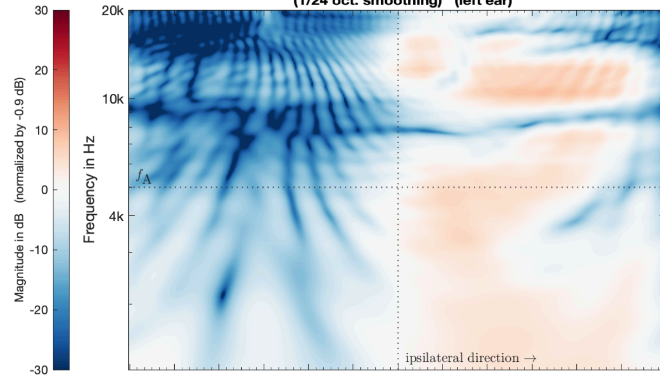
SIM_VSA_EMA17_PW_struct_SubSampled_SH44 -> HRIR_L2702 (1/24 oct. smoothing) (left ear)
