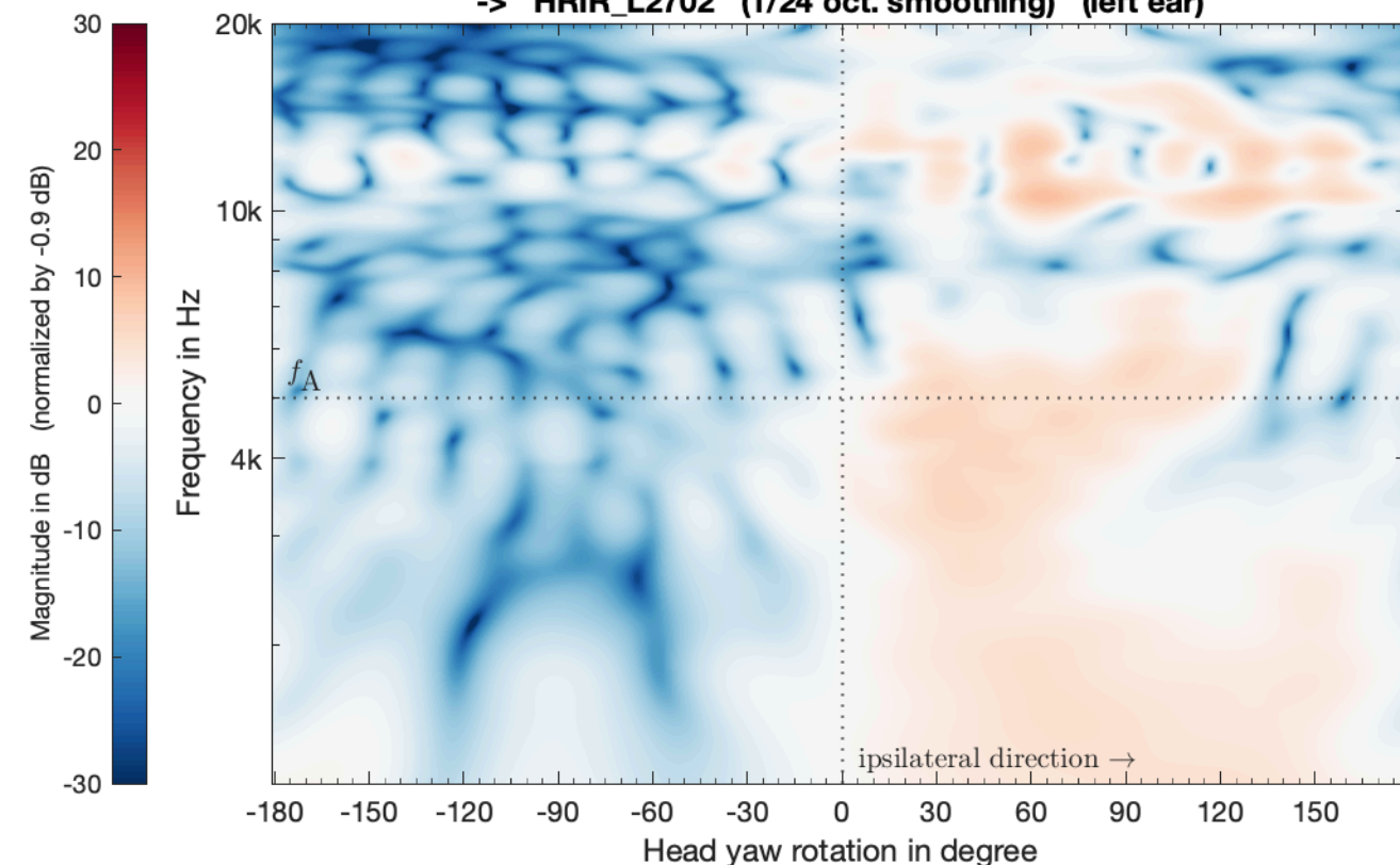
SIM_VSA_EMA17_PW_struct_SubSampled_SH44_eMagLS -> HRIR_L2702 (1/24 oct. smoothing) (left ear)
