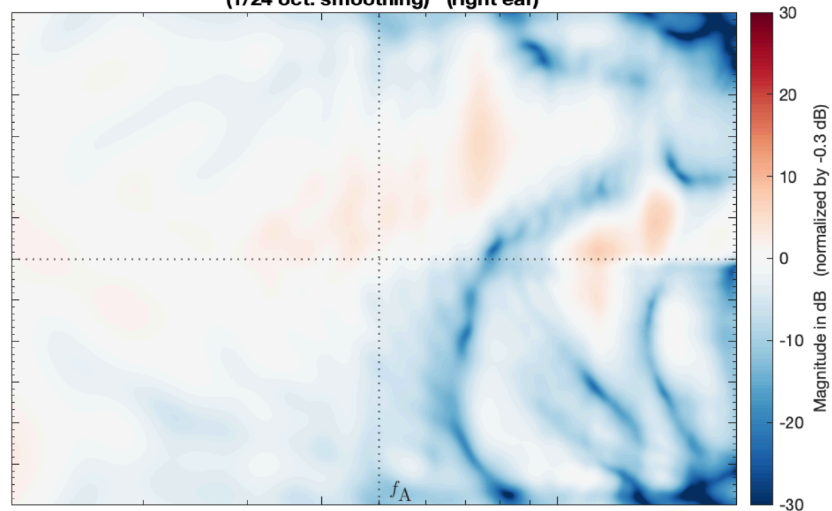
SIM_VSA_EMA17_PW_struct_SubSampled_SH44_eMagLS_vertical -> HRIR_L2702 (1/24 oct. smoothing) (right ear)
