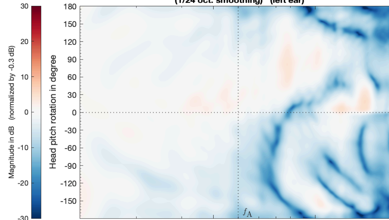
SIM_VSA_EMA17_PW_struct_SubSampled_SH44_vertical -> HRIR_L2702 (1/24 oct. smoothing) (left ear)
