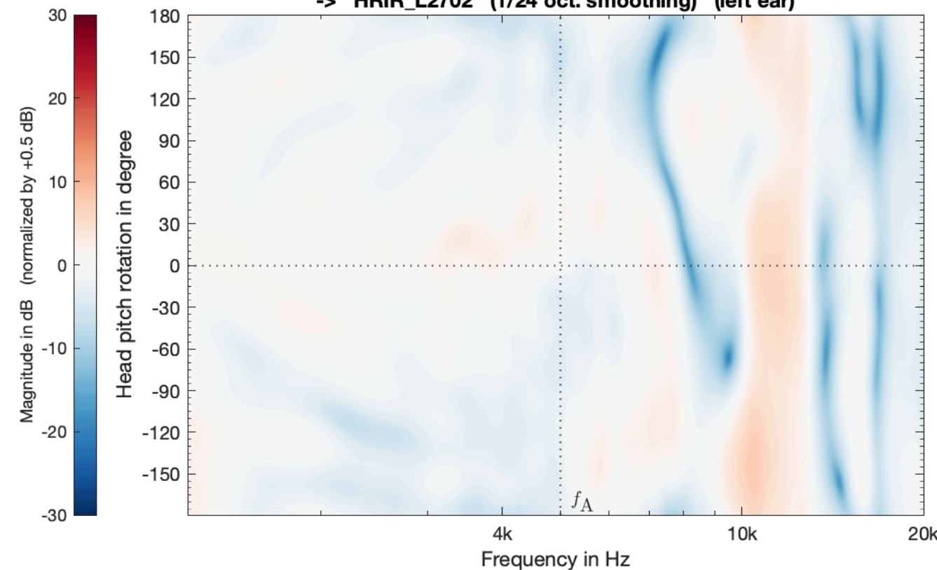
SIM_VSA_EMA17_PW_struct_SubSampled_SH44_vertical -> HRIR_L2702 (1/24 oct. smoothing) (left ear)
