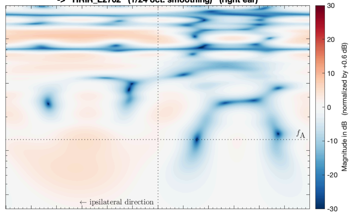
SIM_VSA_EMA5_PW_struct_SubSampled_SH44 -> HRIR_L2702 (1/24 oct. smoothing) (right ear)
