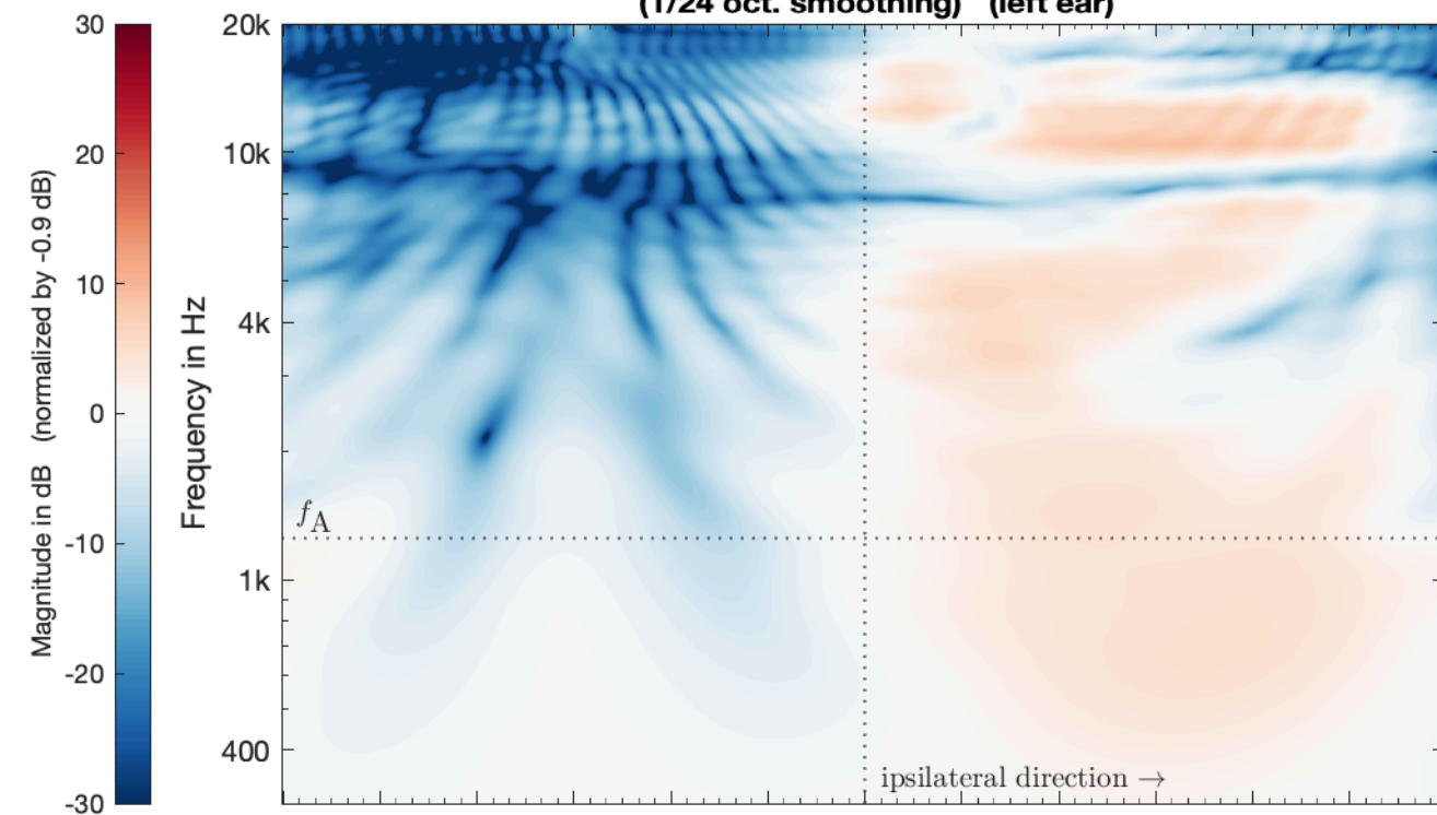
SIM_VSA_EMA5_PW_struct_SubSampled_SH44 -> HRIR_L2702 (1/24 oct. smoothing) (left ear)
