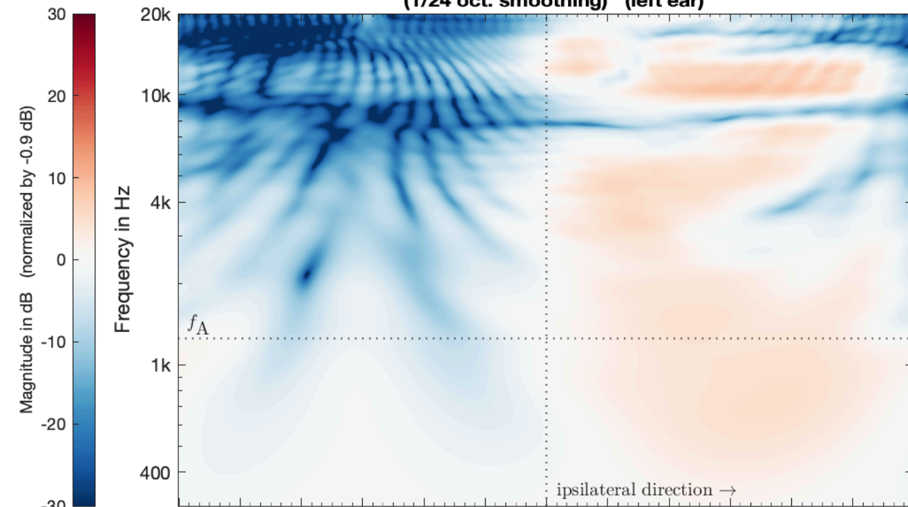
SIM_VSA_EMA5_PW_struct_SubSampled_SH44_eMagLS -> HRIR_L2702 (1/24 oct. smoothing) (left ear)
