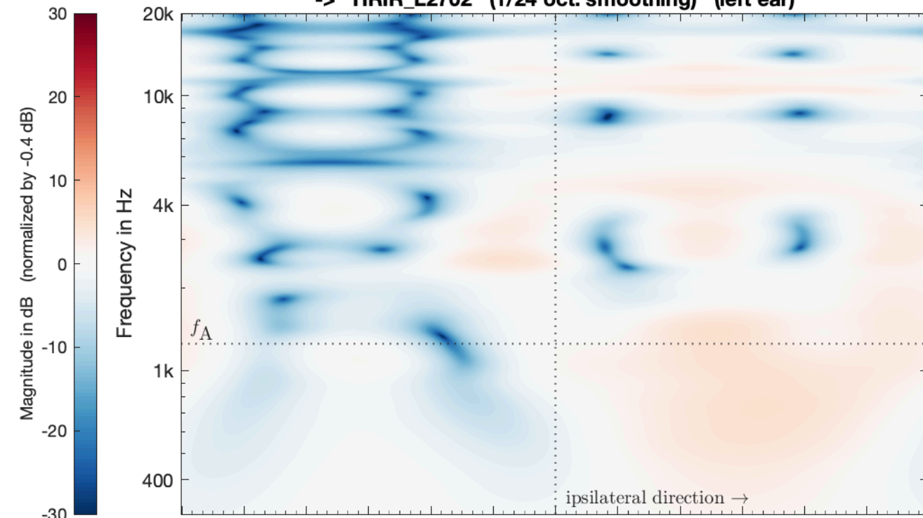
SIM_VSA_EMA5_PW_struct_SubSampled_SH44_eMagLS -> HRIR_L2702 (1/24 oct. smoothing) (left ear)
