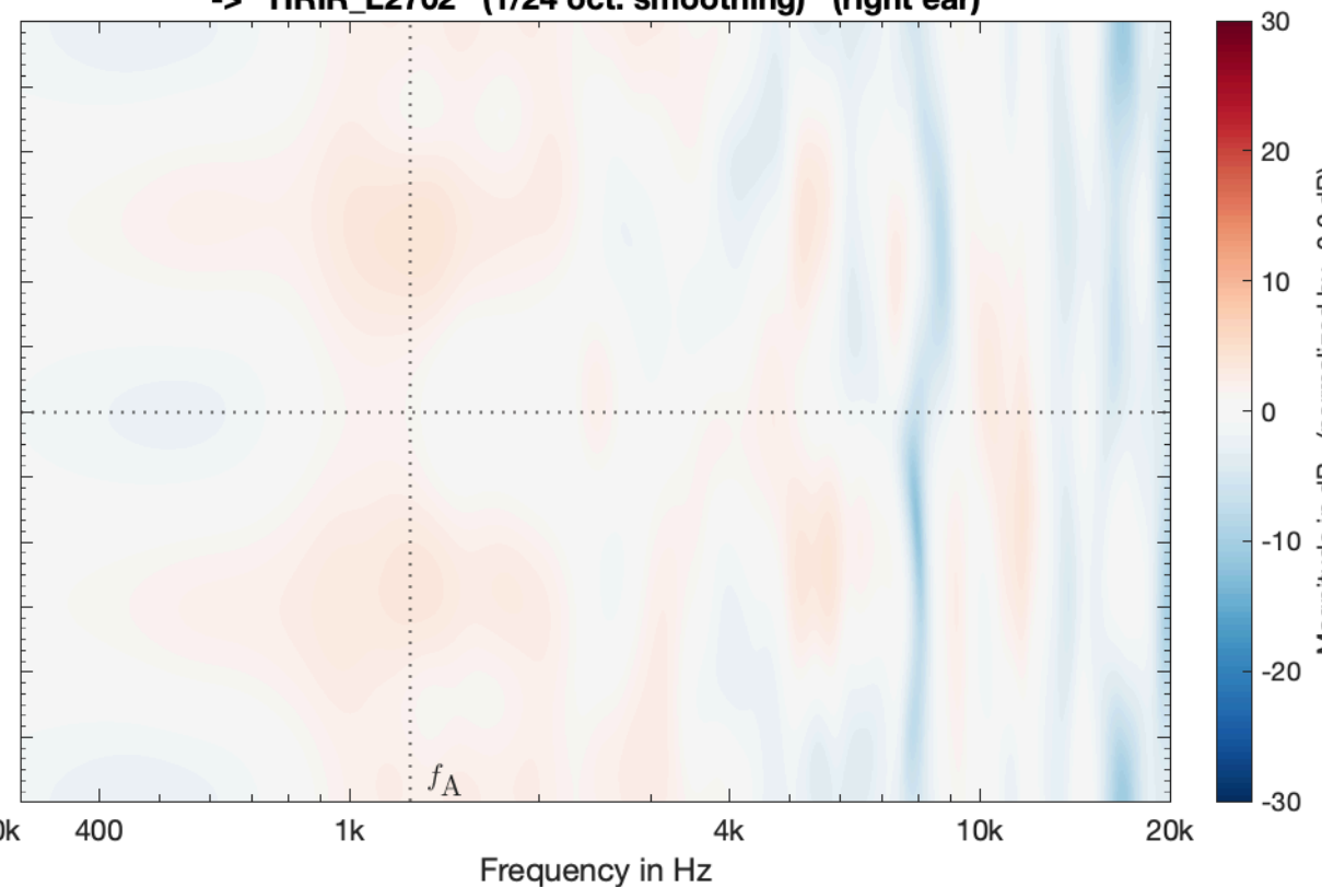
SIM_VSA_EMA5_PW_struct_SubSampled_SH44_eMagLS_vertical -> HRIR_L2702 (1/24 oct. smoothing) (right ear)
