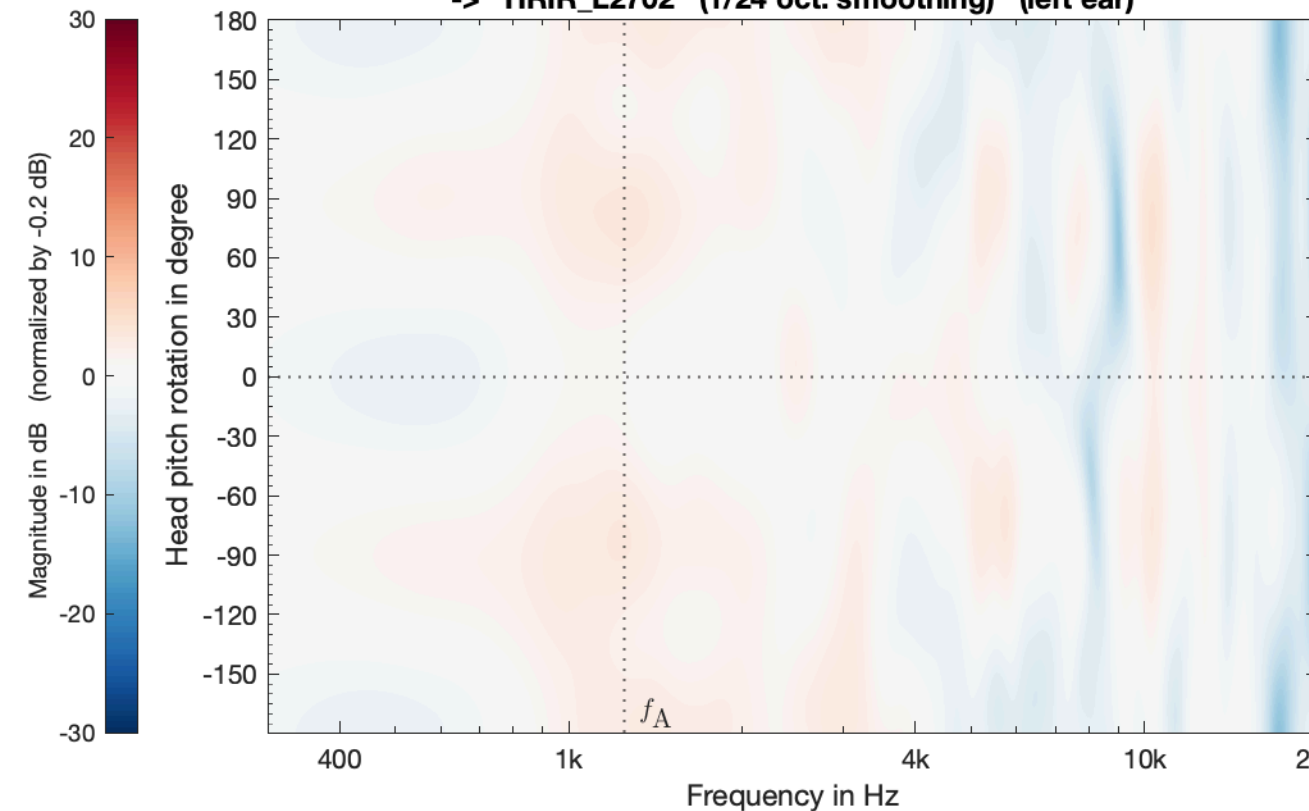
SIM_VSA_EMA5_PW_struct_SubSampled_SH44_eMagLS_vertical -> HRIR_L2702 (1/24 oct. smoothing) (left ear)
