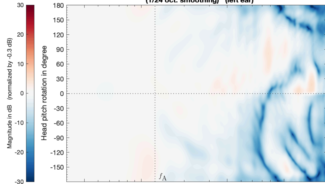
SIM_VSA_EMA5_PW_struct_SubSampled_SH44_eMagLS_vertical -> HRIR_L2702 (1/24 oct. smoothing) (left ear)
