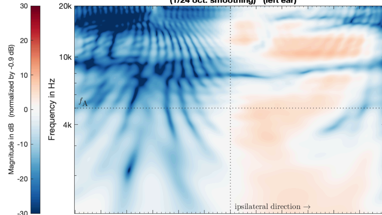
SIM_VSA_SMA_TD146_PW_struct_SubSampled_SH44_eMagLS -> HRIR_L2702 (1/24 oct. smoothing) (left ear)
