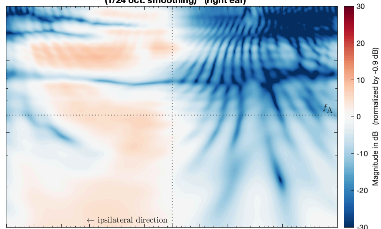
SIM_VSA_SMA_TD146_PW_struct_SubSampled_SH44_eMagLS -> HRIR_L2702 (1/24 oct. smoothing) (right ear)
