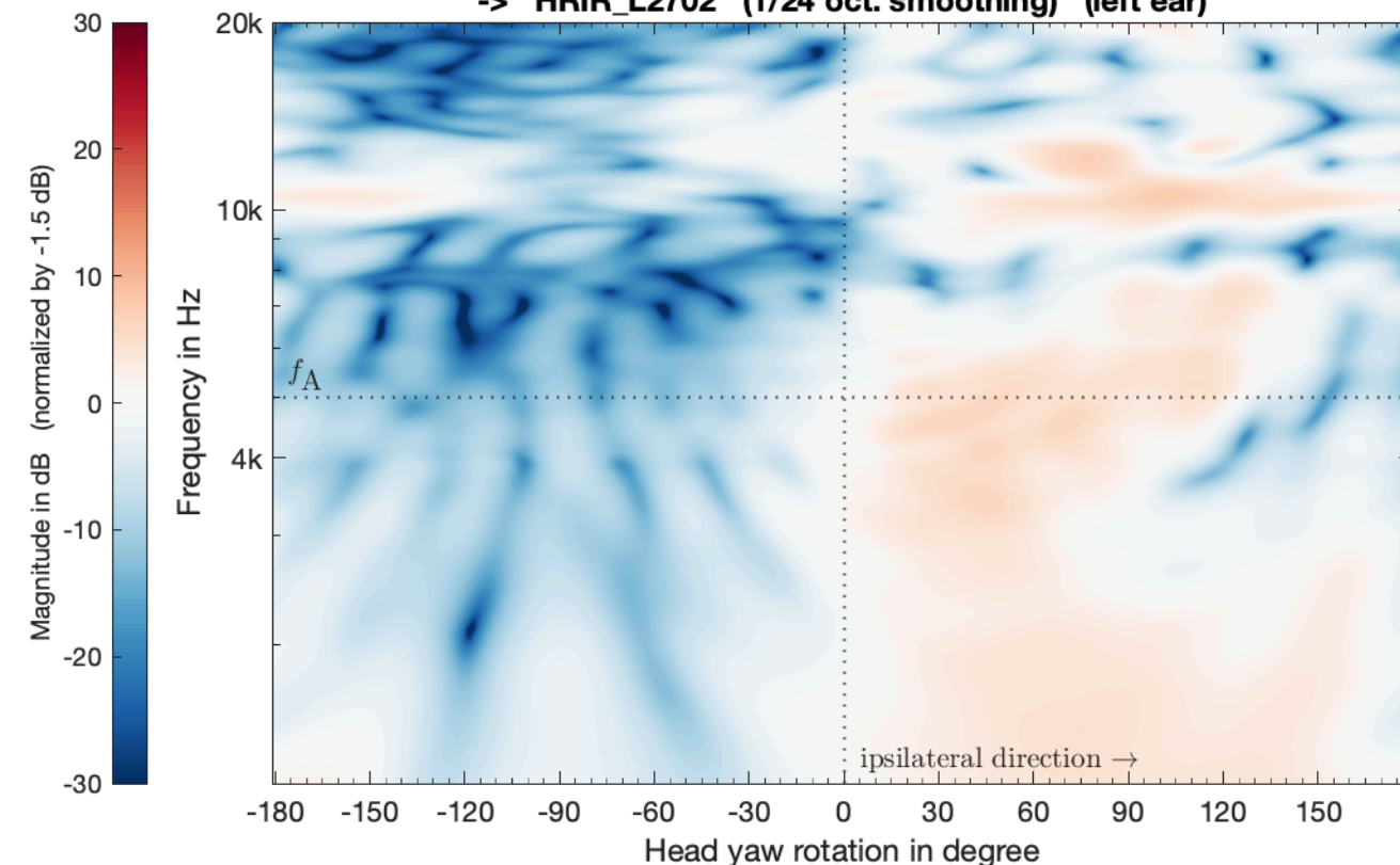
SIM_VSA_SMA_TD146_PW_struct_SubSampled_SH44_eMagLS -> HRIR_L2702 (1/24 oct. smoothing) (left ear)
