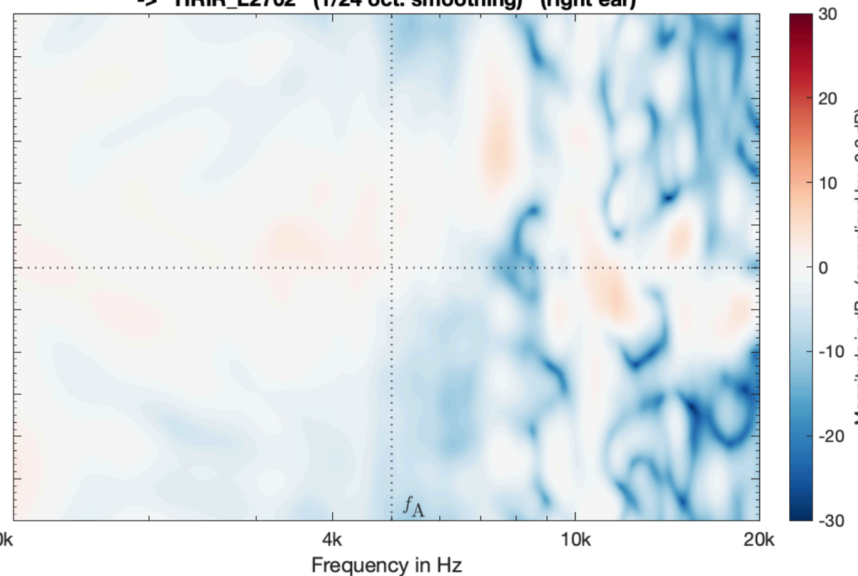
SIM_VSA_SMA_TD146_PW_struct_SubSampled_SH44_eMagLS_vertical -> HRIR_L2702 (1/24 oct. smoothing) (right ear)
