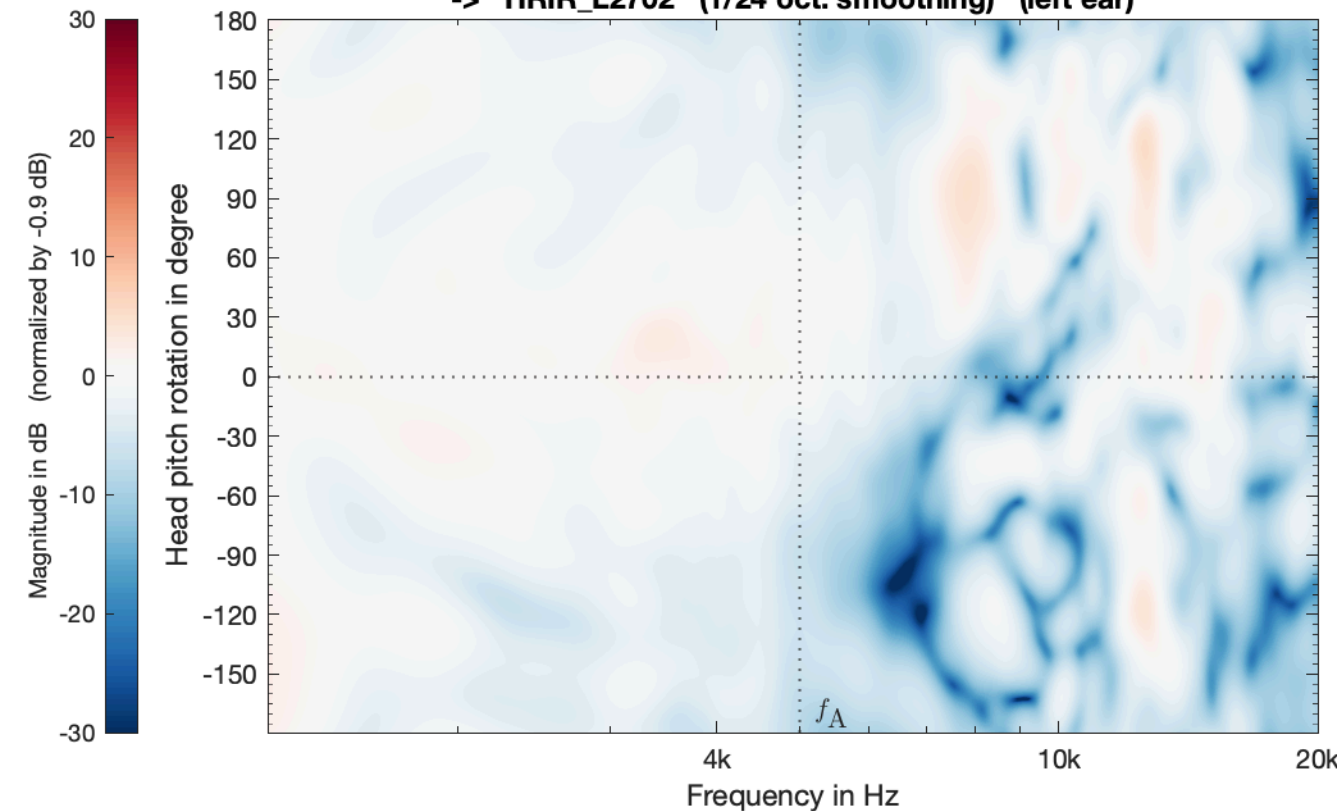
SIM_VSA_SMA_TD146_PW_struct_SubSampled_SH44_eMagLS_vertical -> HRIR_L2702 (1/24 oct. smoothing) (left ear)
