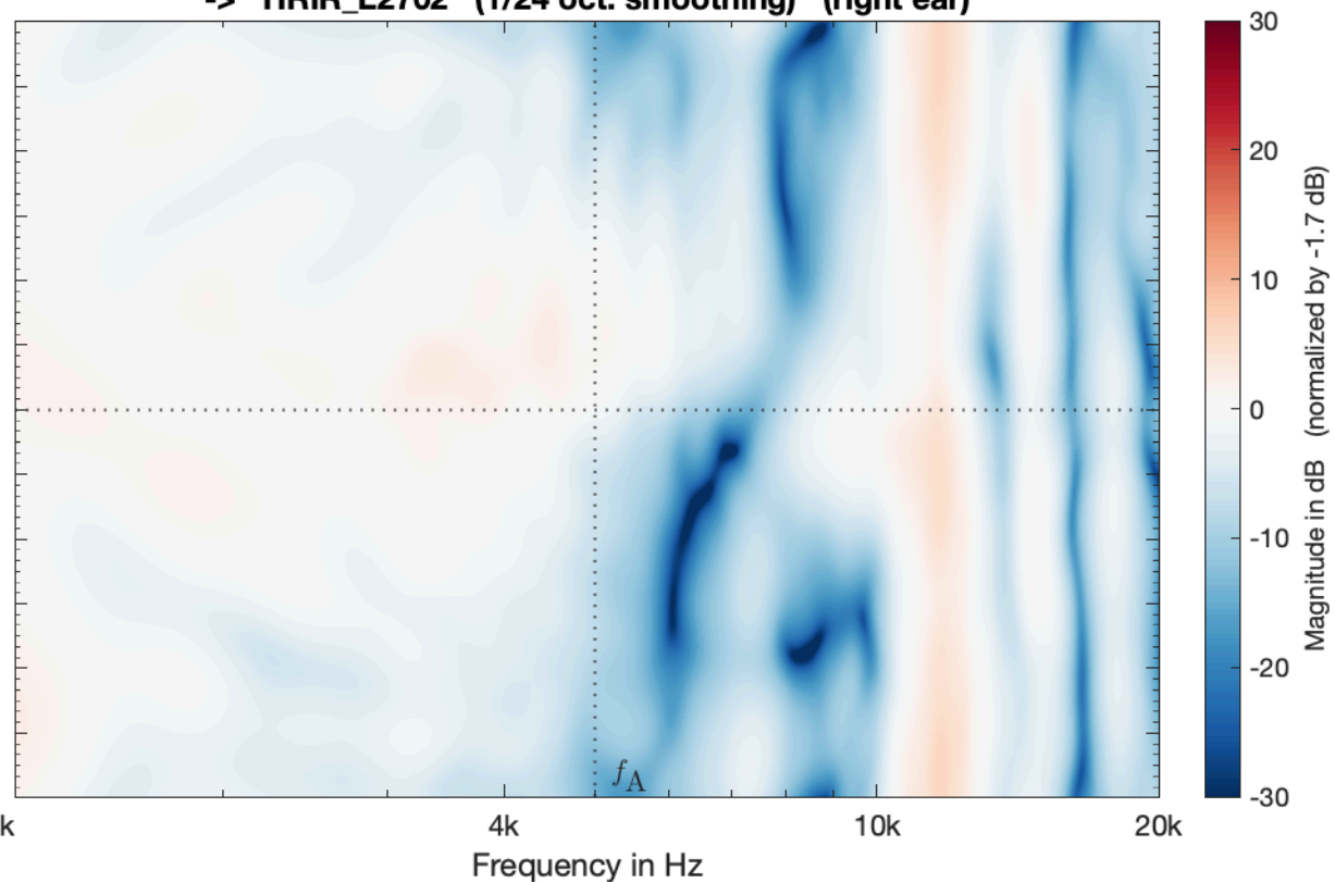
SIM_VSA_SMA_TD146_PW_struct_SubSampled_SH44_vertical -> HRIR_L2702 (1/24 oct. smoothing) (right ear)
