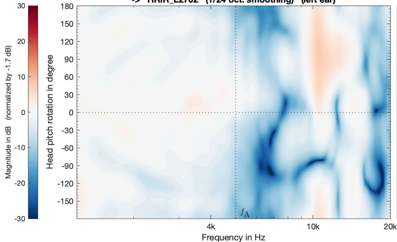
SIM_VSA_SMA_TD146_PW_struct_SubSampled_SH44_vertical -> HRIR_L2702 (1/24 oct. smoothing) (left ear)
