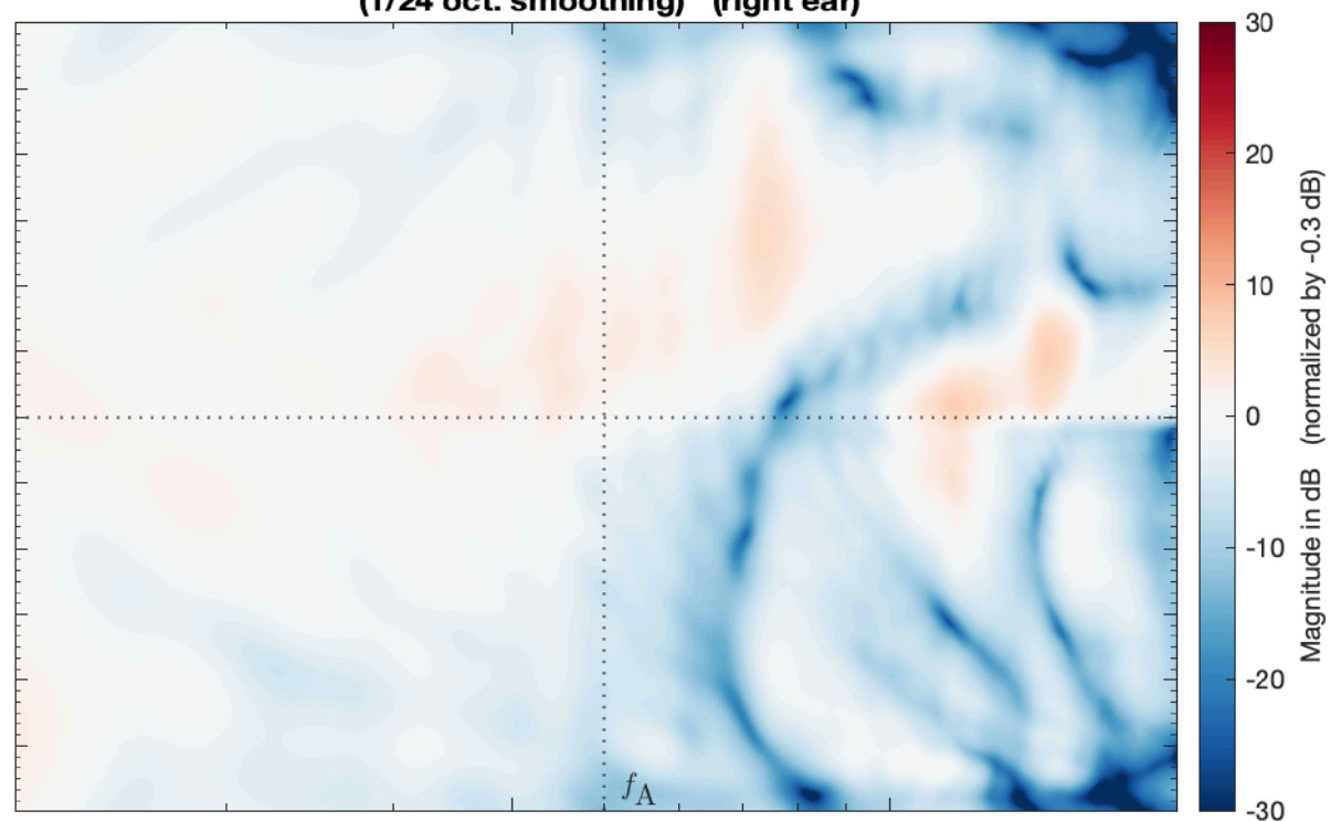
SIM_VSA_SMA_TD146_PW_struct_SubSampled_SH44_vertical -> HRIR_L2702 (1/24 oct. smoothing) (right ear)
