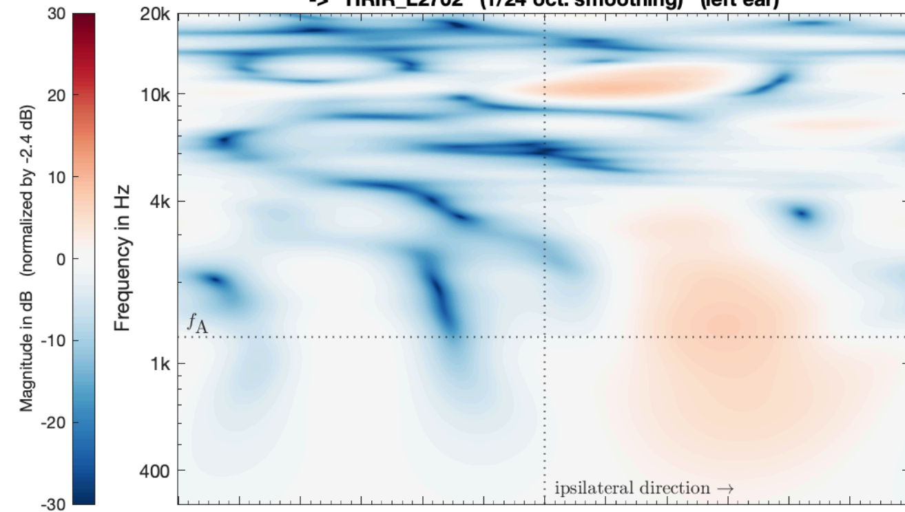
SIM_VSA_SMA_TD14_PW_struct_SubSampled_SH44 -> HRIR_L2702 (1/24 oct. smoothing) (left ear)
