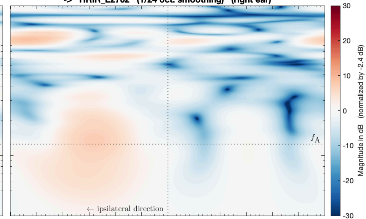
SIM_VSA_SMA_TD14_PW_struct_SubSampled_SH44 -> HRIR_L2702 (1/24 oct. smoothing) (right ear)
