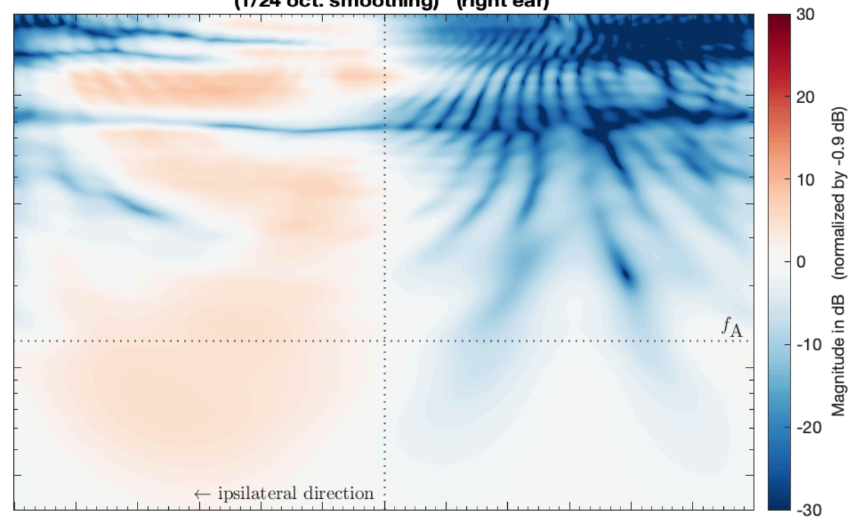
SIM_VSA_SMA_TD14_PW_struct_SubSampled_SH44 -> HRIR_L2702 (1/24 oct. smoothing) (right ear)
