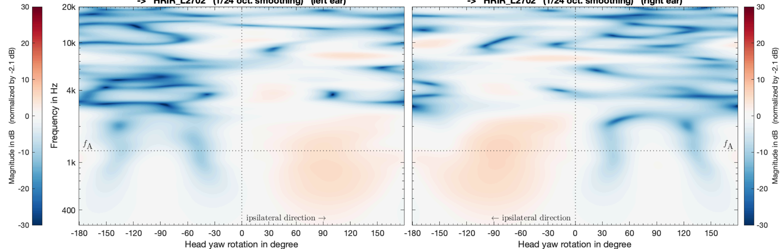
SIM_VSA_SMA_TD14_PW_struct_SubSampled_SH44_eMagLS -> HRIR_L2702 (1/24 oct. smoothing) (left ear)
