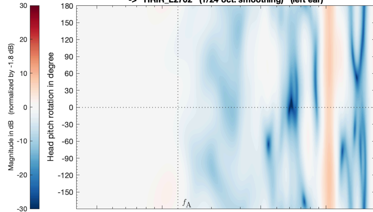
SIM_VSA_SMA_TD14_PW_struct_SubSampled_SH44_vertical -> HRIR_L2702 (1/24 oct. smoothing) (left ear)
