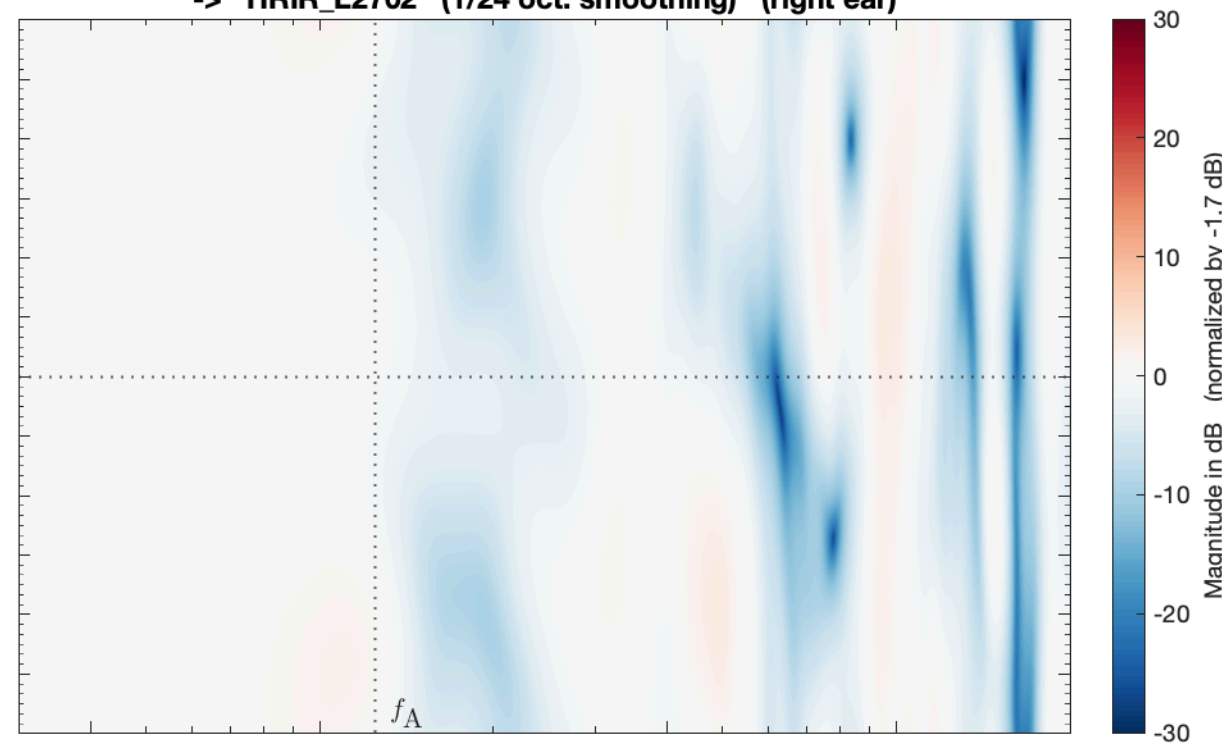
SIM_VSA_SMA_TD14_PW_struct_SubSampled_SH44_vertical -> HRIR_L2702 (1/24 oct. smoothing) (right ear)
