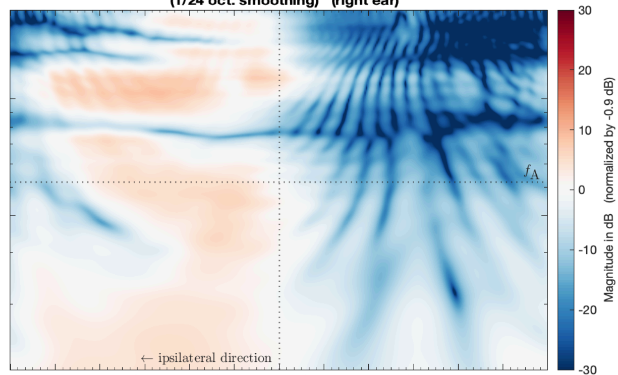
Simulation_SMA_EM32_SrcEar_eMagLS -> HRIR_L2702 (1/24 oct. smoothing) (right ear)
