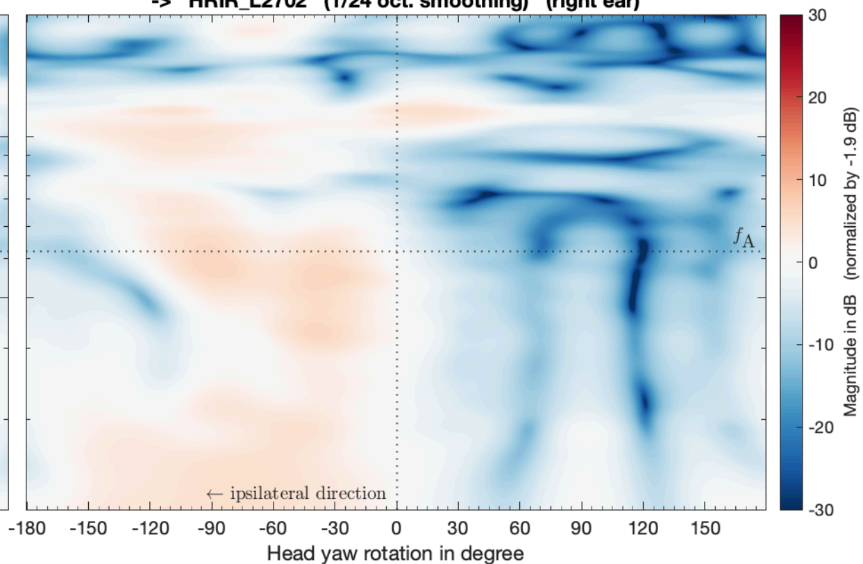
Simulation_SMA_EM32_SrcEar_eMagLS -> HRIR_L2702 (1/24 oct. smoothing) (right ear)
