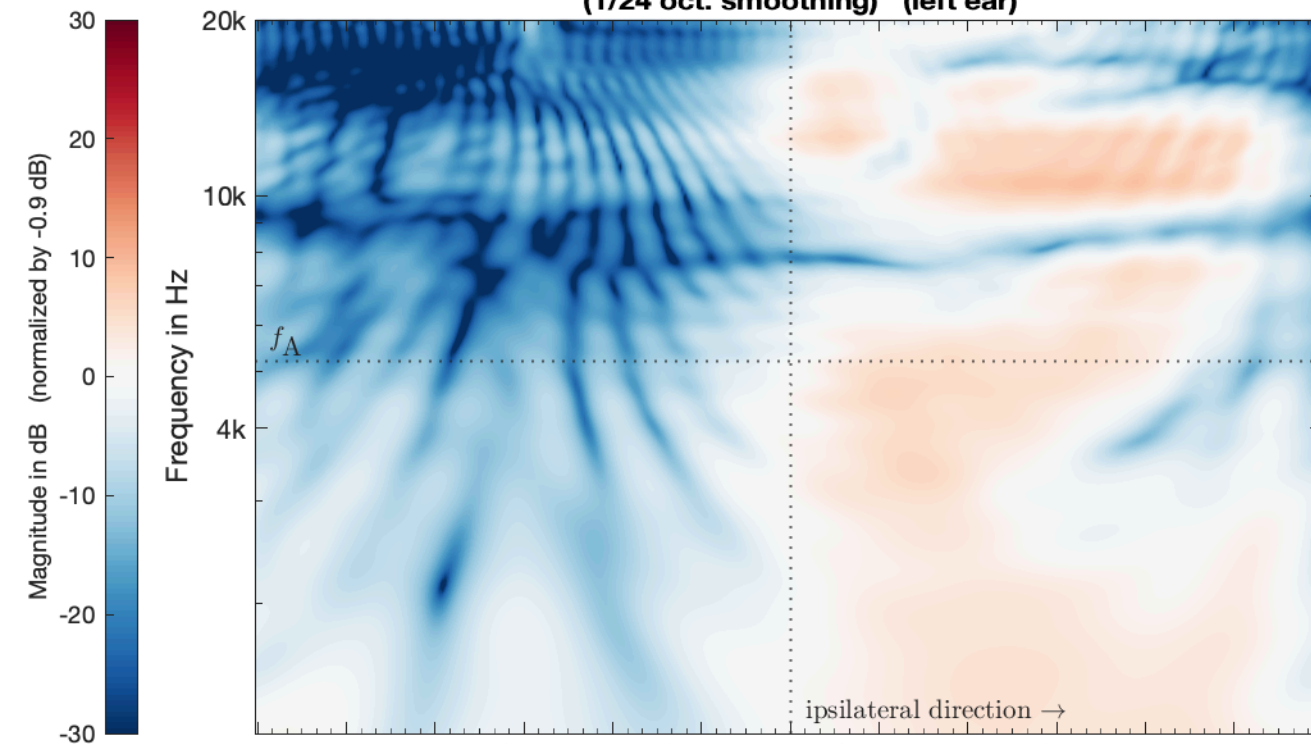
Simulation_SMA_EM32_SrcEar_eMagLS -> HRIR_L2702 (1/24 oct. smoothing) (left ear)
