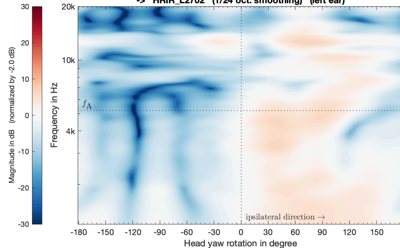
Simulation_SMA_EM32_SrcEar_eMagLS -> HRIR_L2702 (1/24 oct. smoothing) (left ear)
