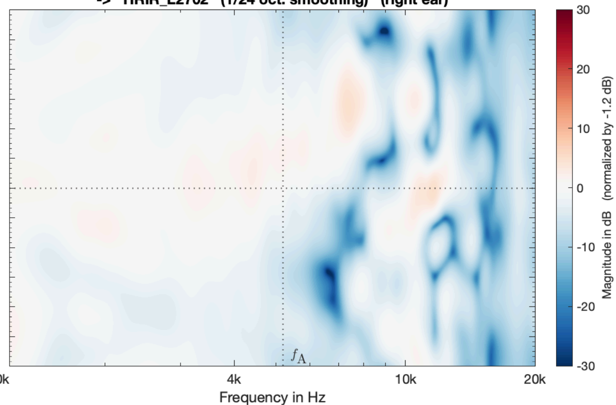
Simulation_SMA_EM32_SrcEar_eMagLS_vertical -> HRIR_L2702 (1/24 oct. smoothing) (right ear)
