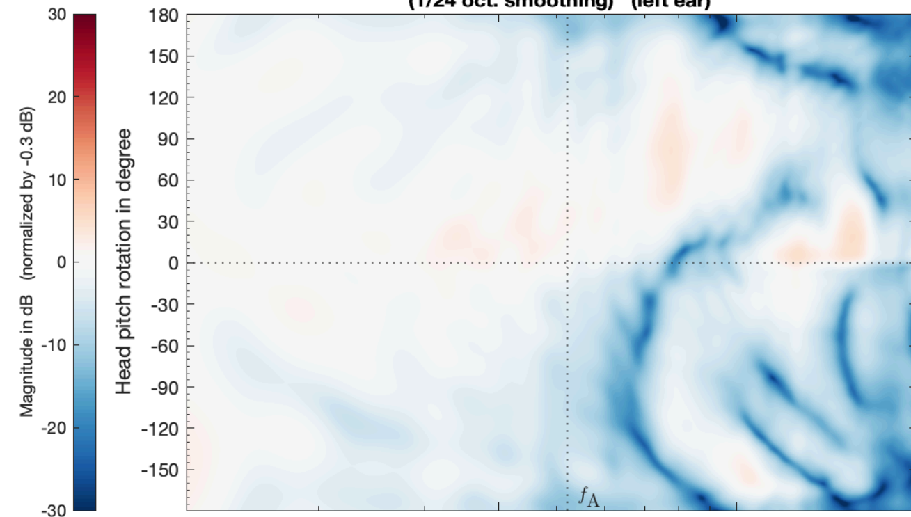
Simulation_SMA_EM32_SrcEar_eMagLS_vertical -> HRIR_L2702 (1/24 oct. smoothing) (left ear)
