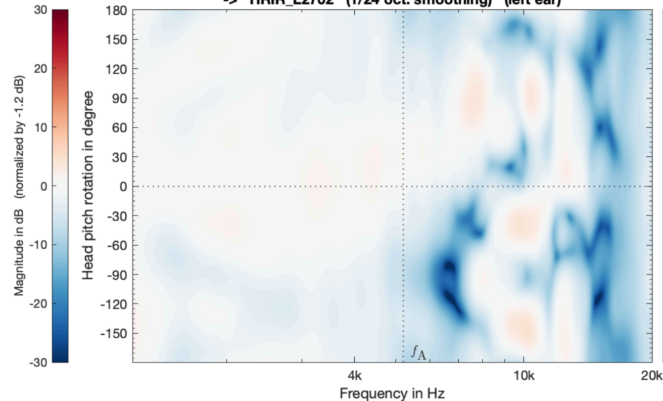
Simulation_SMA_EM32_SrcEar_eMagLS_vertical -> HRIR_L2702 (1/24 oct. smoothing) (left ear)
