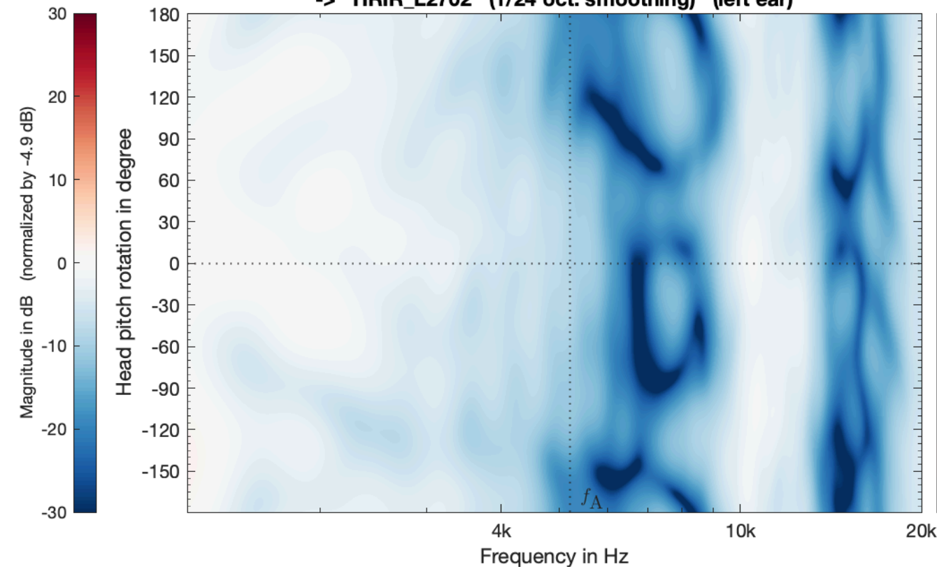
Simulation_SMA_EM32_SrcEar_vertical -> HRIR_L2702 (1/24 oct. smoothing) (left ear)
