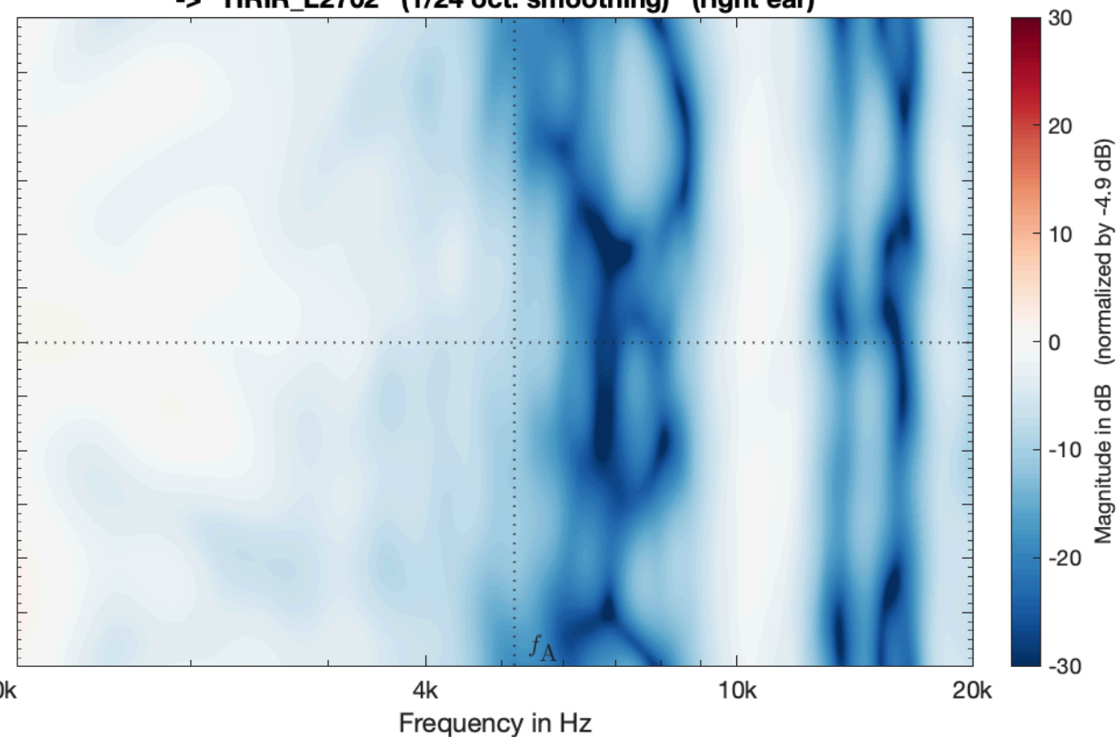
Simulation_SMA_EM32_SrcEar_vertical -> HRIR_L2702 (1/24 oct. smoothing) (right ear)
