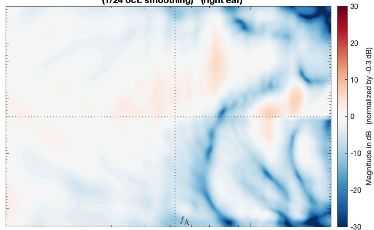
Simulation_SMA_EM32_SrcEar_vertical -> HRIR_L2702 (1/24 oct. smoothing) (right ear)
