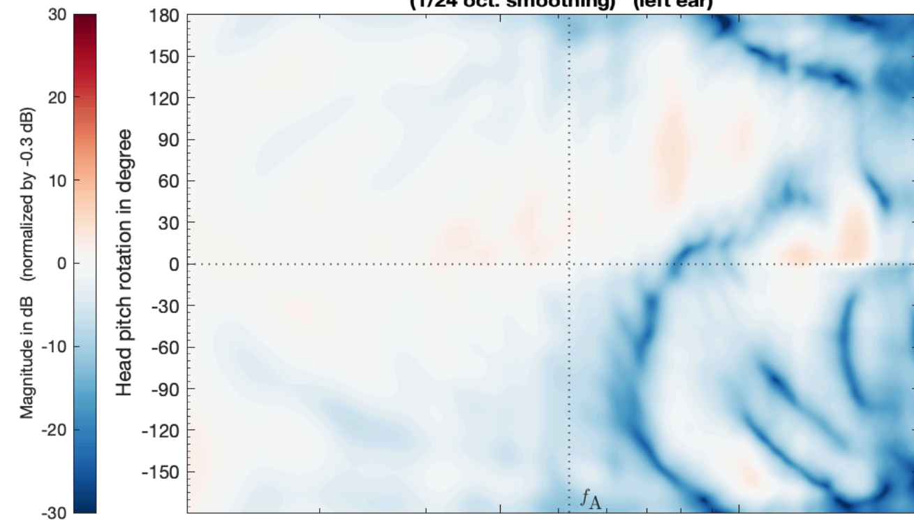
Simulation_SMA_EM32_SrcEar_vertical -> HRIR_L2702 (1/24 oct. smoothing) (left ear)
